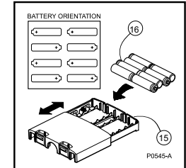
Figure 10 - Replacing the Battery Lid
